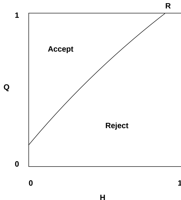
Figure 3: Accept and Reject Regions in Howard [2002] Model
