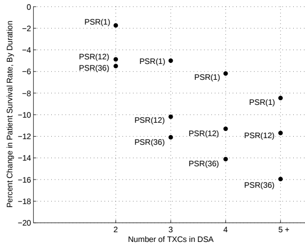
Figure 13: LS Percentage Change in Patient Survival Rates, by Duration and Number of transplant centers in Donation Service Area
