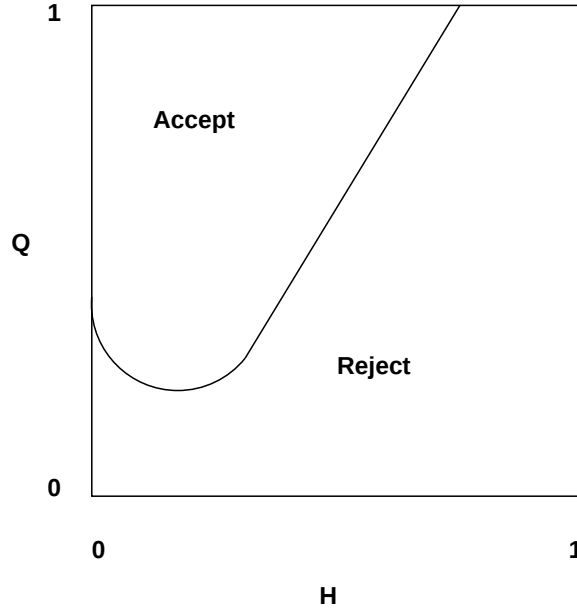
Figure 4: Alternative Accept and Reject Regions
