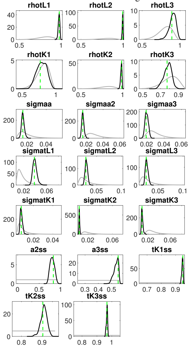
Figure 11: Priors and Posteriors
