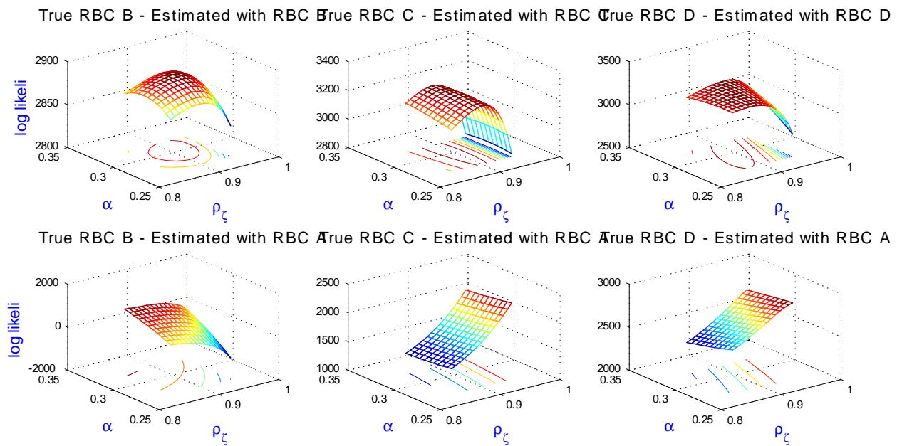
Figure 3: Likelihood surfaces
