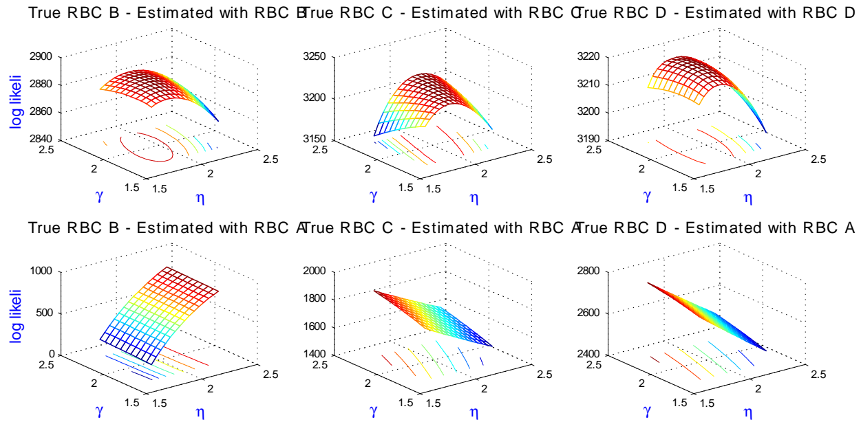
Figure 2: Likelihood surfaces
