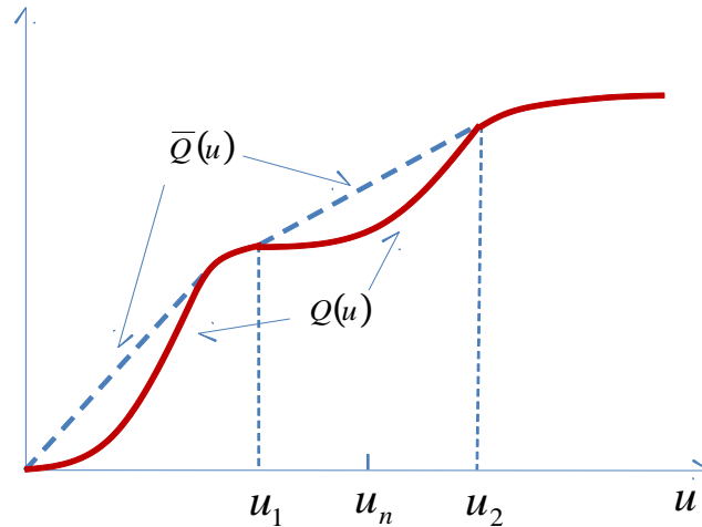
Figure 2: Convex envelope
