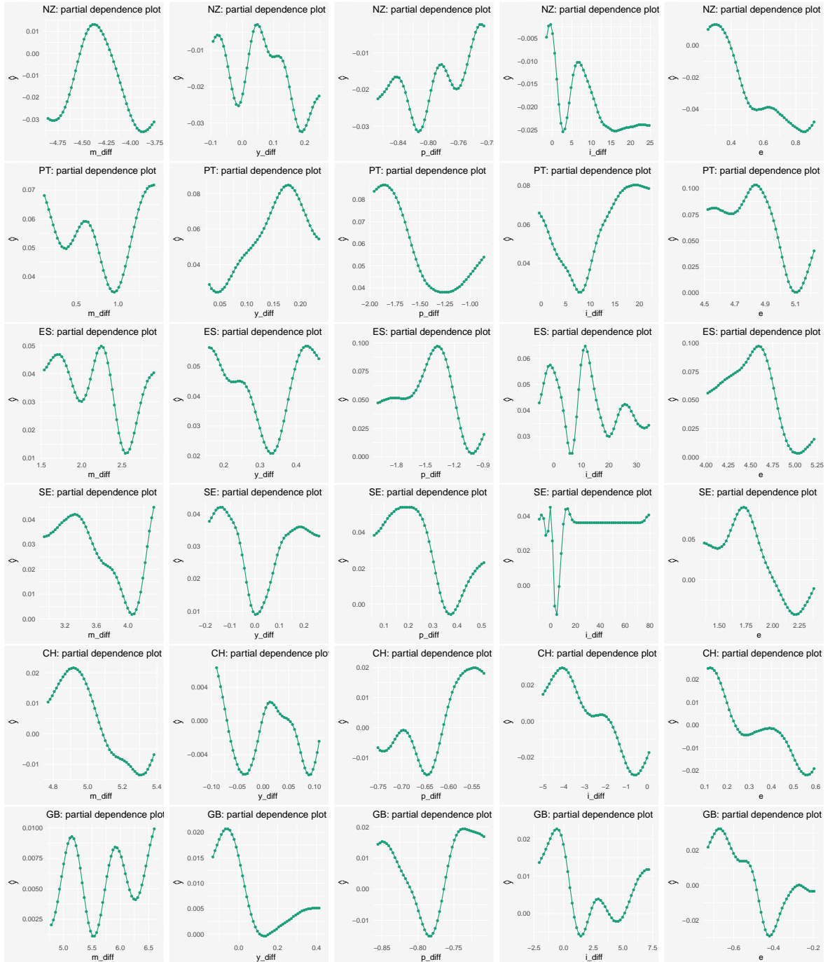
Figure 25: Partial dependence plots, 12 months ahead forecasts, SVM.
