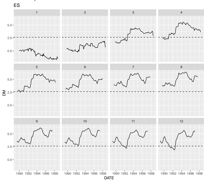
Figure 11: Fluctuation test. Monetary model with sticky prices and UIP deviations, 1 to 12 months ahead forecasts, SVM.
