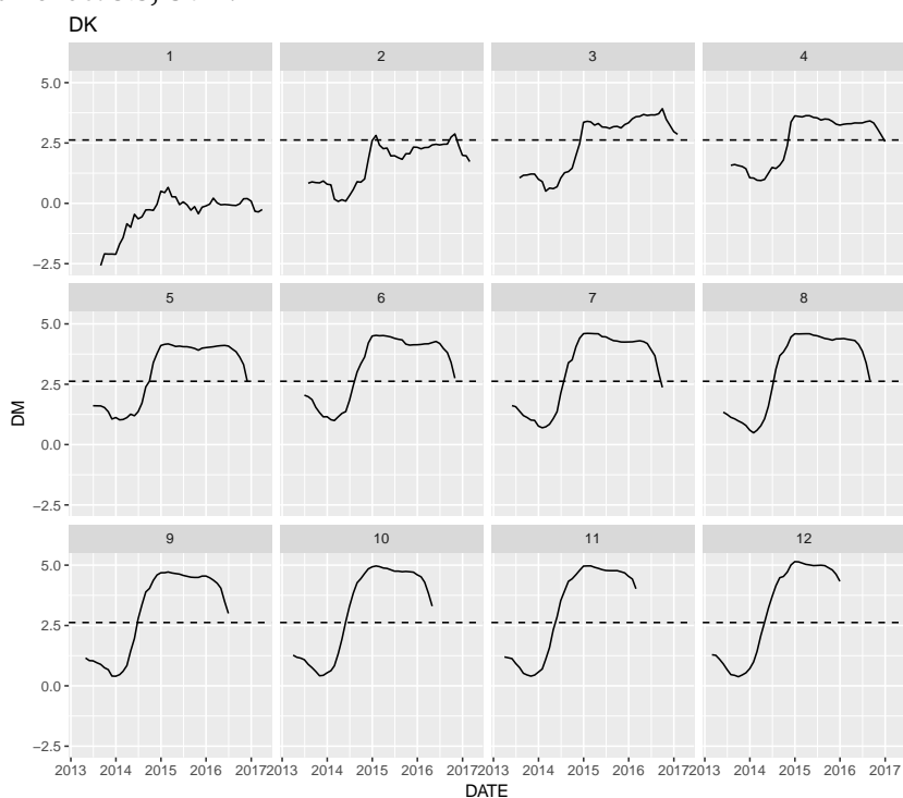
Figure 10: Fluctuation test. Monetary model with sticky prices and UIP deviations, 1 to 12 months ahead forecasts, SVM.
