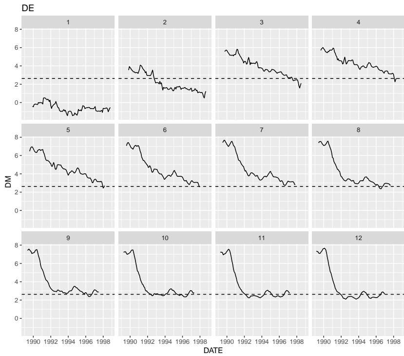
Figure 9: Fluctuation test. Monetary model with sticky prices and UIP deviations, 1 to 12 months ahead forecasts, SVM.
