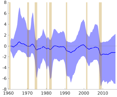
Figure 8: g_t (Model I)
