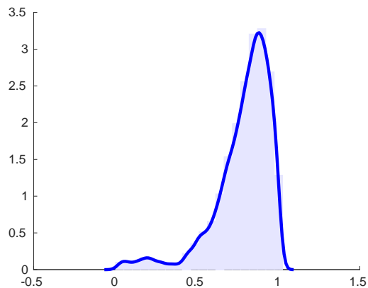
Figure 4: Posterior of \rho_g
