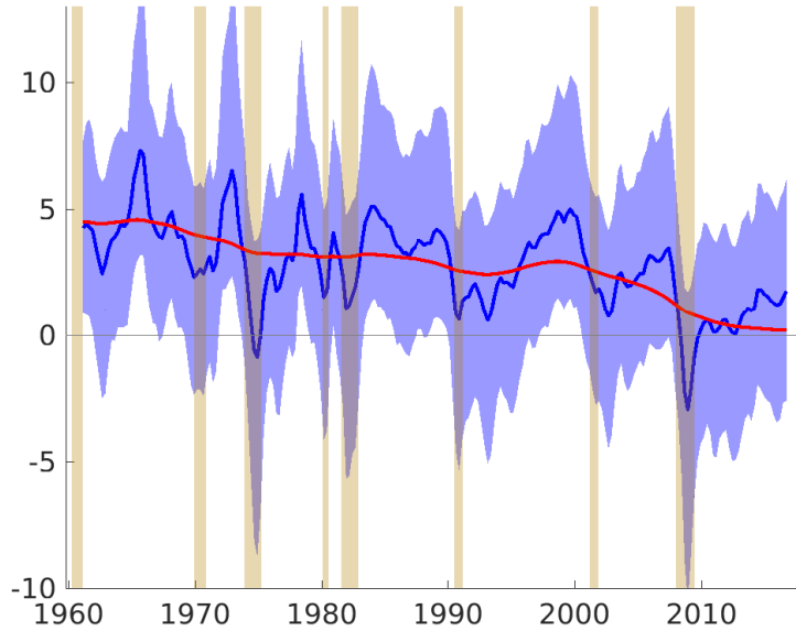
Figure 5: r^* Path (Model III)
