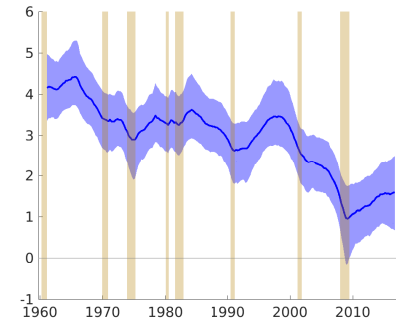
Figure 9: g_t (Model III)
