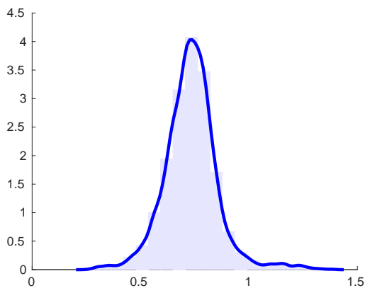
Figure 3: Posterior of \mu_g
