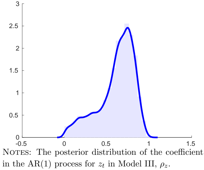
Figure 10: Posterior of \rho_z
