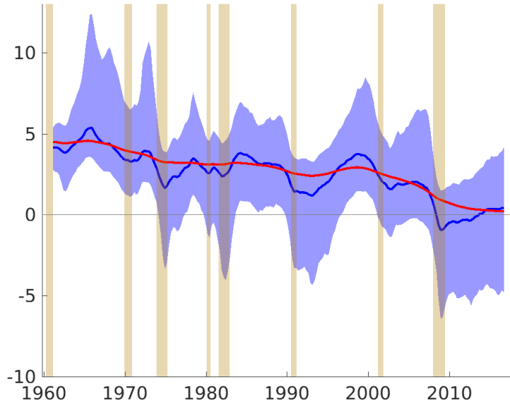
Figure 1: r^* Path (Model I)
