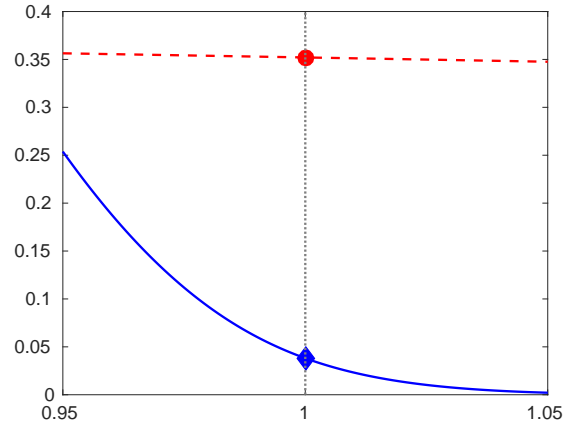
Figure 13: Area around \rho_z = 1
