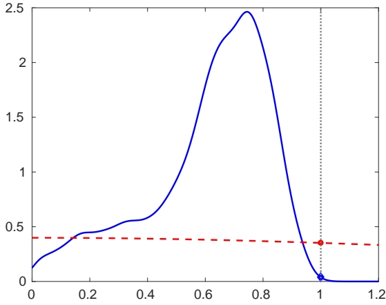
Figure 12: Prior and Posterior of \rho_z
