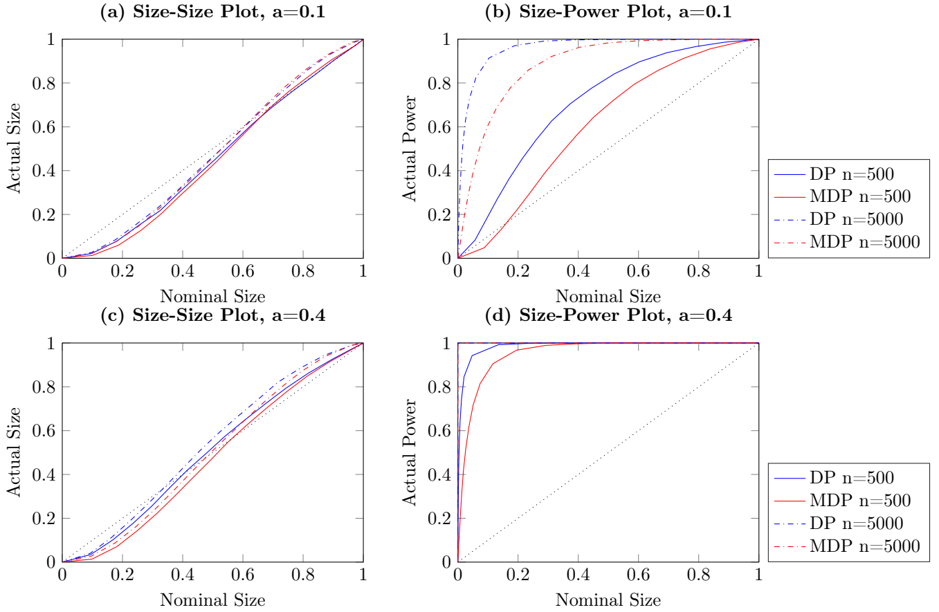
Figure 6: Size-size and size-power plots of Granger non-causality tests, based on 5,000 replications. The DGP is bivariate ARCH as in eq. (20), with Y affecting X . The left (right) column shows observed rejection rates under the null(alternative), blue color stands for DP test while red line indicates modified DP test. Real line and dash line present results with sample size n = 500 and n = 5000 , respectively.
