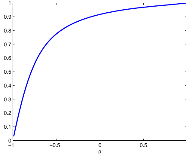
Figure 9: plim(\hat{\lambda}) for different values of \rho
