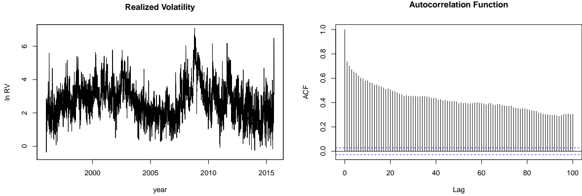
Figure 5: Daily log-realized variances of the S&P500 index and their autocorrelation function.
