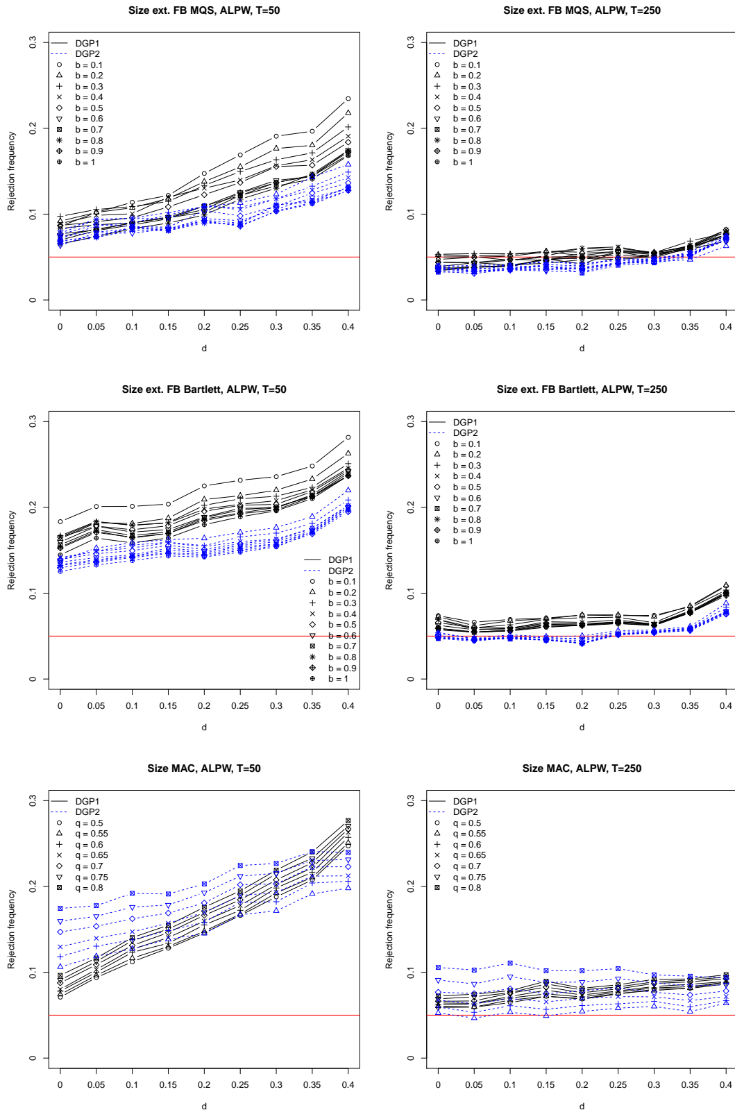
Figure 8: Size of the t_{MAC} and t_{EFB} statistics for different degrees of long memory d , sample sizes T and bandwidth parameters q and b , if the ALPW estimator is used for the plug-in estimation of d .
