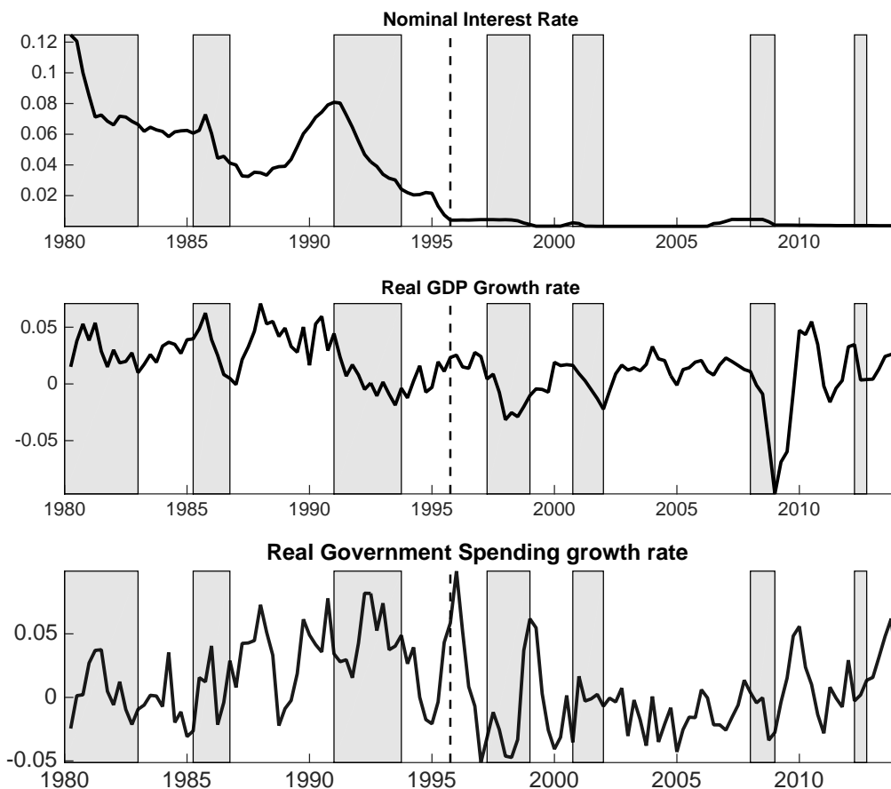
Figure 1: Japan 1980Q2-2014Q1
