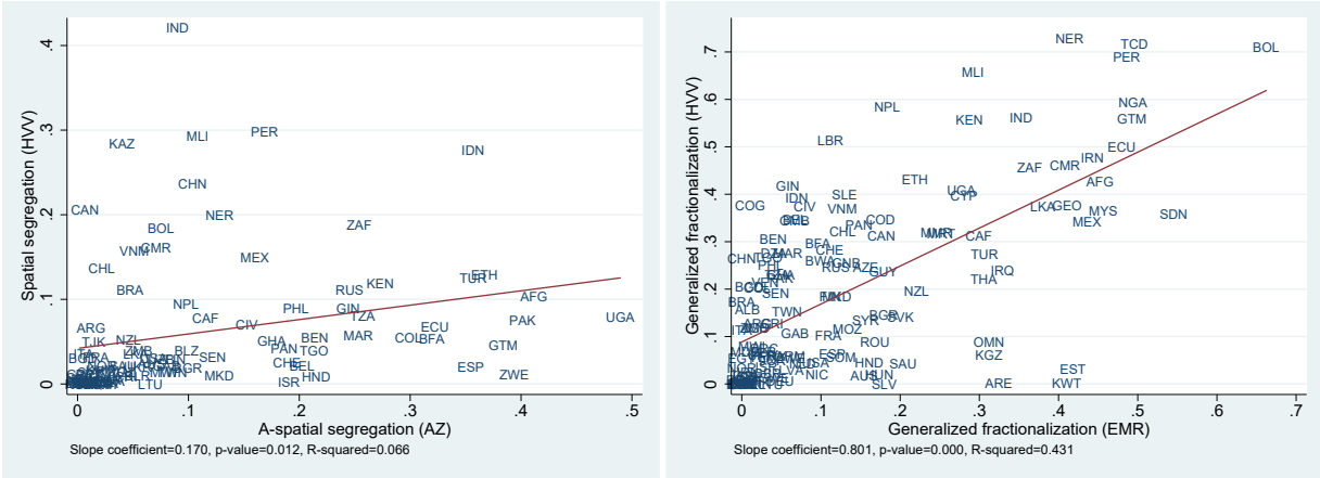
Figure 5: Scatter plots illustrating the relation between our indices and alternative indices
