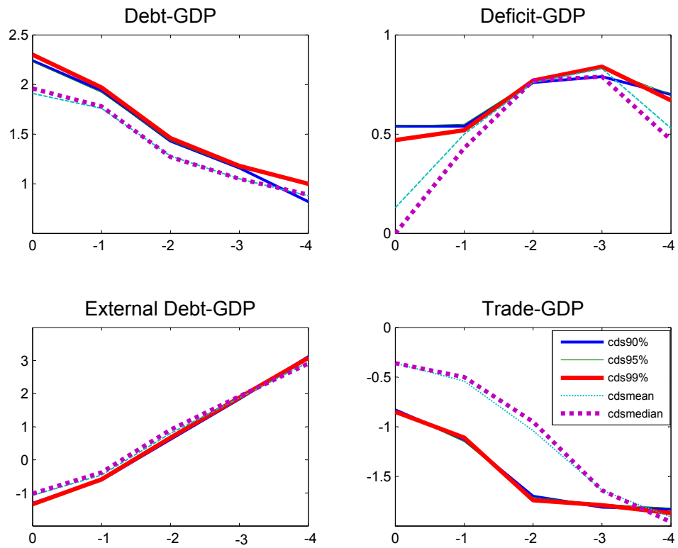
Figure 9: T-Statistics
