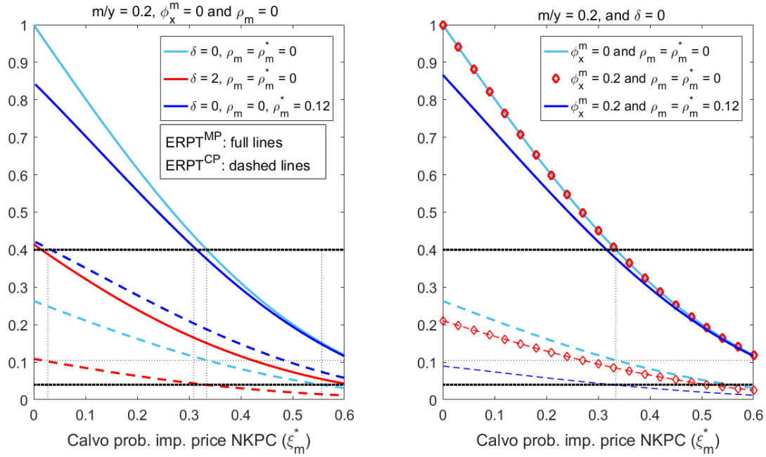
Figure 4: Illustration of Corollaries C1-C4 for sticky import prices for EA ( \frac{\bar{m}}{\bar{c}+\bar{i}} = 0.26 )
