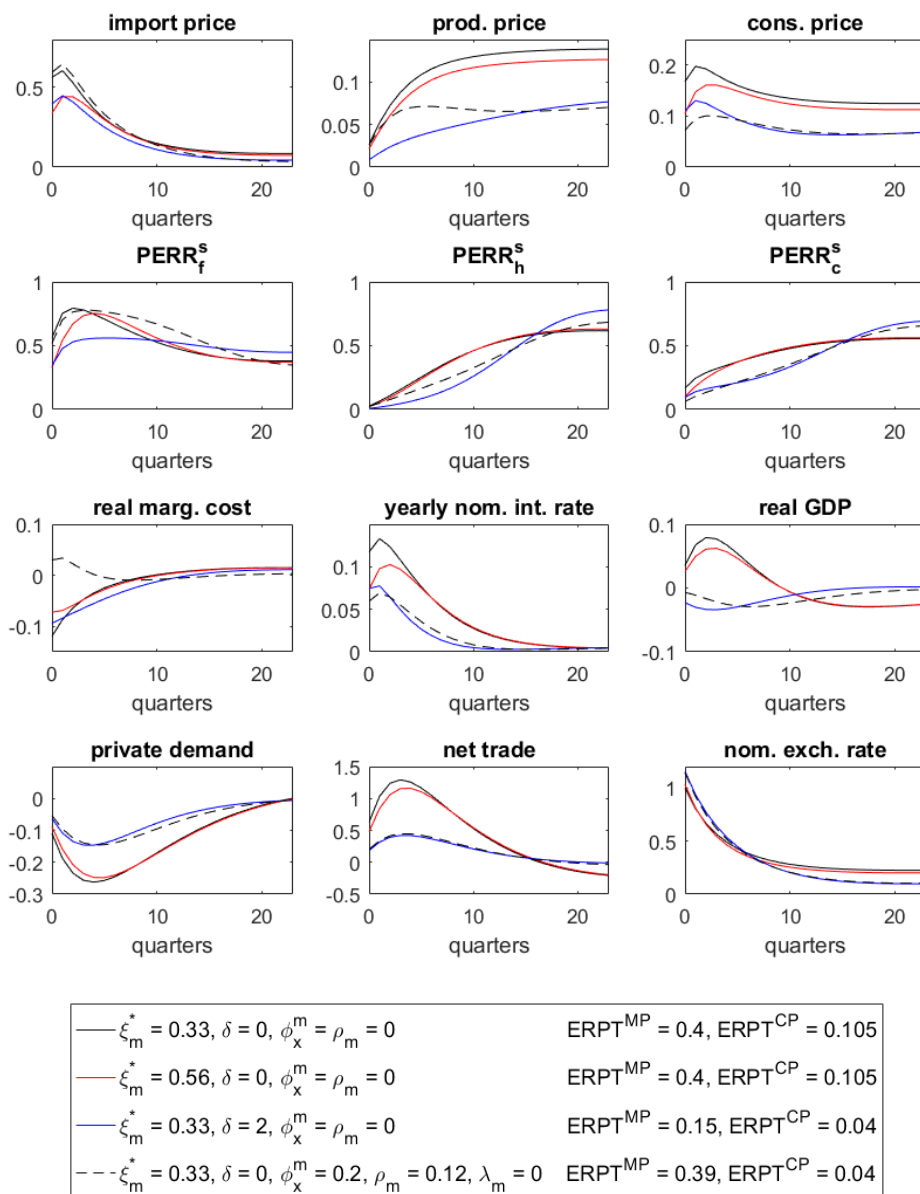
Figure 6: Impulse responses to a UIP shock
