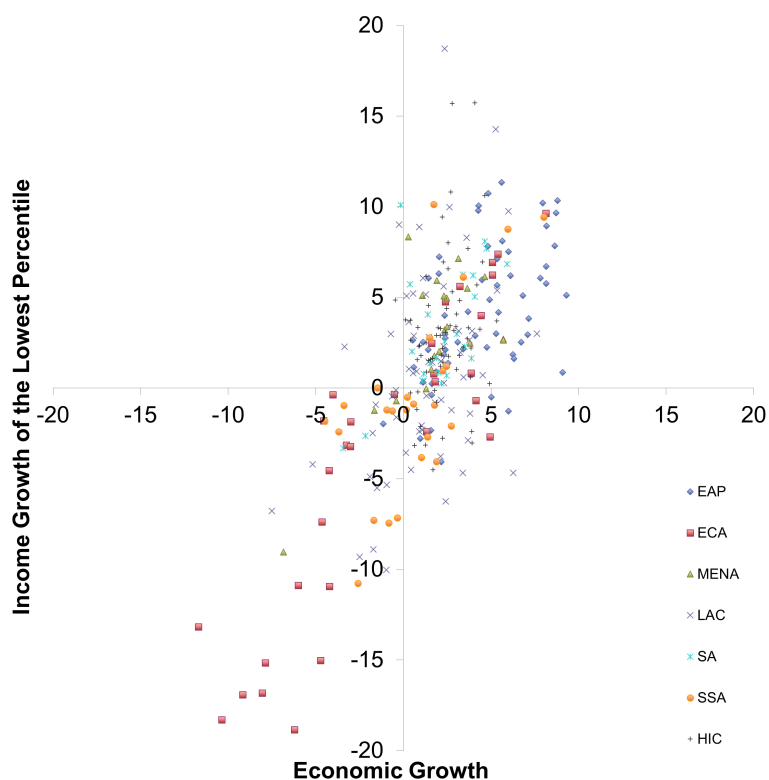
Figure 4: Geographic Decomposition
