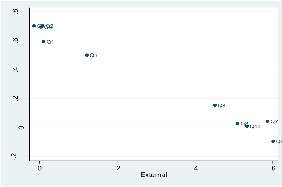
Figure 3: Cross-plot of factor loadings of the items from Rotter (1966) scale.
