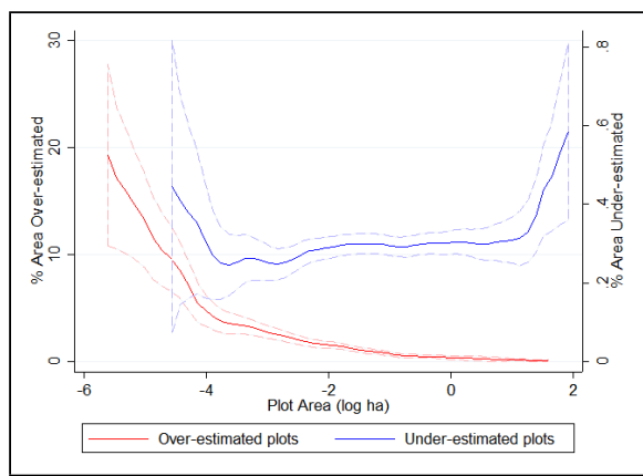
Figure A2: Plot Size Perception Error over Plot Size
