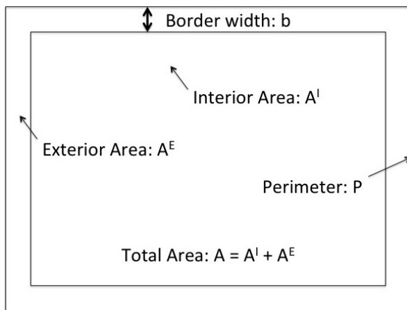
Figure 1: Plot Area Schematic
