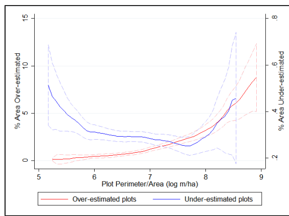
Figure A3: Plot Size Perception Error over Perimeter-Area Ratio
