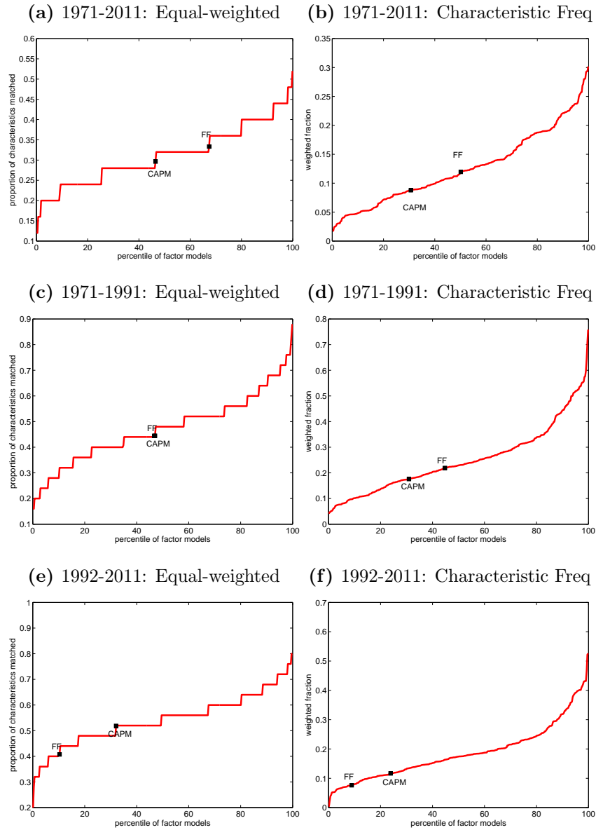
Figure C.1 displays the distribution of three-factor model performance, as measured by the percentage of characteristics matched, over the whole sample period 1971-2011 and subsamples 1971-1991 and 1992-2011. The universe of factor models is all three-factor models consisting of the market portfolio and two characteristic return factors from our list of 27. Factors are the high minus low portfolio from sorting the largest 80% of firms into ten portfolios with respect to the underlying firm characteristic. The percentage of characteristics matched is computed using two characteristic weighting methods: equal-weighted method and characteristic matching frequency method. The “equal-weighted” method gives an equal weight to each characteristic matched. The “characteristic matching frequency” method gives each characteristic a weight of 1 minus the proportion of factor models that can match the cross-section of returns based on the characteristic under consideration. For comparison, the figures also show the rankings of the CAPM and the Fama-French three-factor model.
